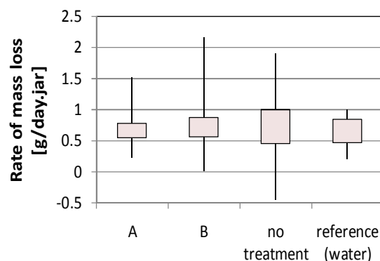
Figure 3: Box and whisker plot of mass loss rate showing 95% confidence region (box) and min and max values (whisker)
